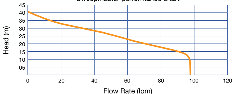
Sweepmaster performance chart
